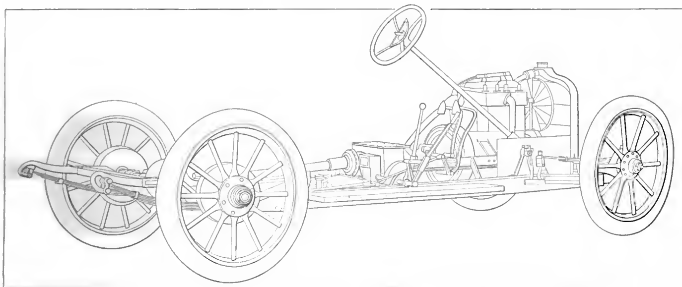
Fig. 3—Three-quarter view of the American chassis, showing the underslung feature, the method of suspension and the sub-frame, carrying the motor and transmission
